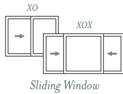
Sliding Window
